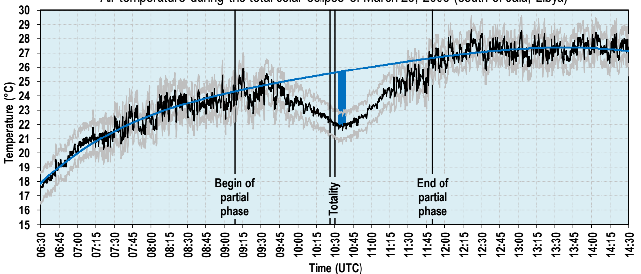
Air temperature during the total solar eclipse of March 29, 2006 (south of Jalu, Libya)
