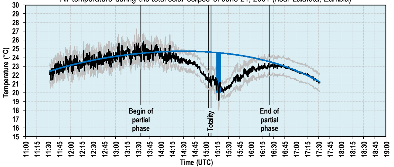
Air temperature during the total solar eclipse of June 21, 2001 (near Lalafuta, Zambia)
